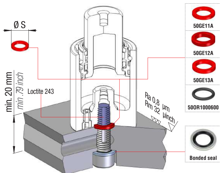
Example thread size M8 x 12
