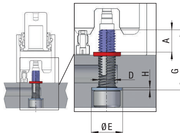
Example thread size M8 x 12
