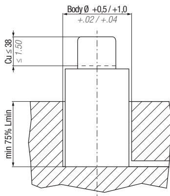
Installation in a flat-end hole.
