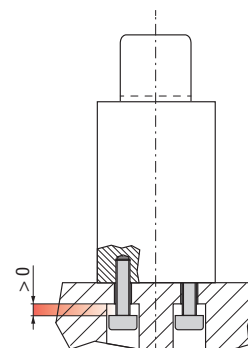
Installation NOT allowed due to incorrect screw length.
